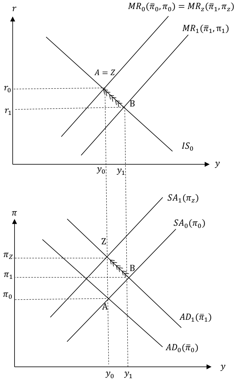
Figure 11 Rising target inflation: the transition toward steady-state equilibrium
