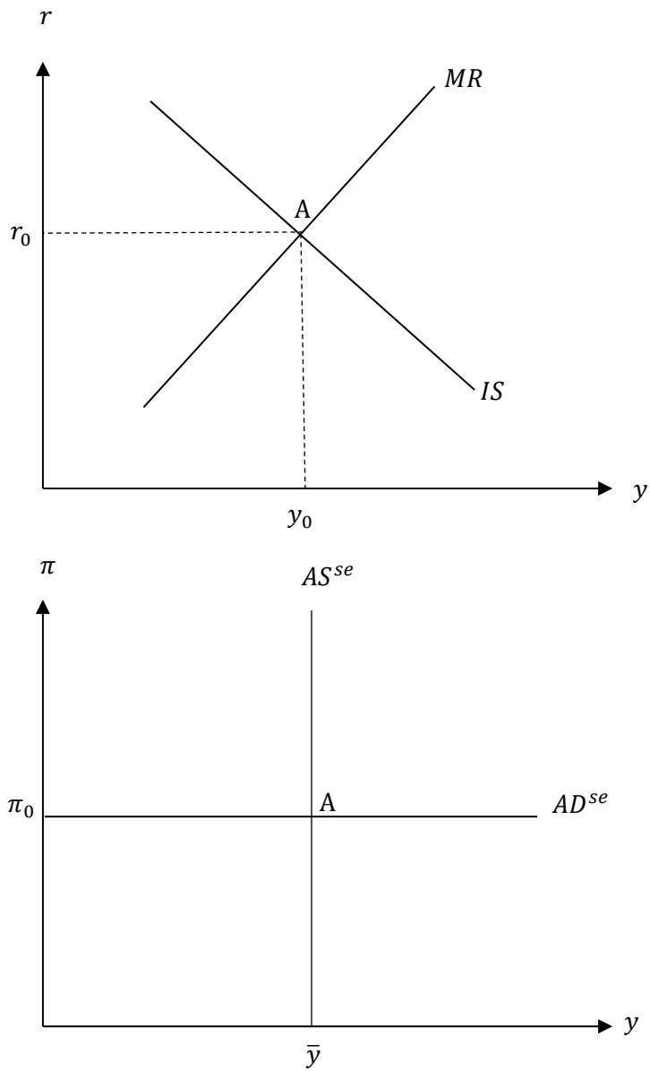
Figure 9 Steady-state general equilibrium
