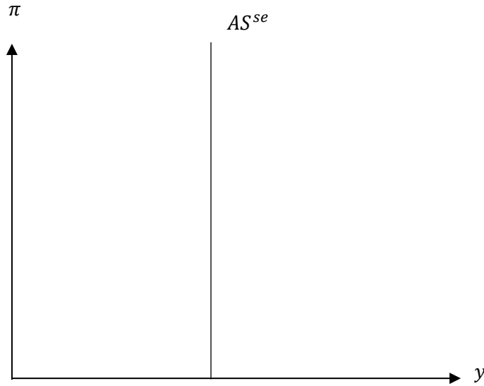
Figure 7 Steady-state equilibrium aggregate supply
