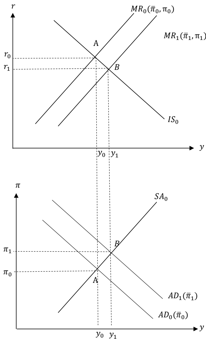
Figure 10 Rising target inflation: the short term
